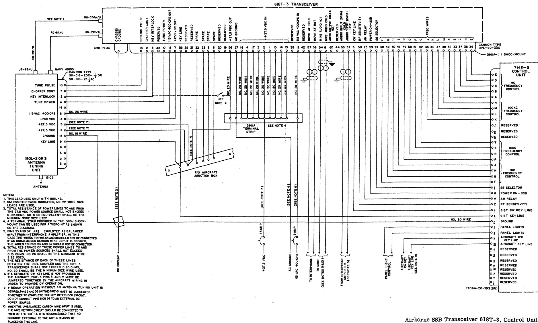
Airborne SSB Transceiver 618T-3, Control Unit 714E-3, and Antenna Tuner 180L-2 ( ), Interconnecting Wiring Diagram Figure 123
