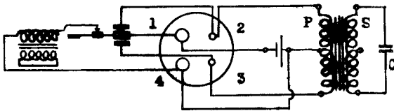
Series-driven vibrator type N.S.
