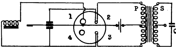
Shunt-driven vibrator type N.S.B.
