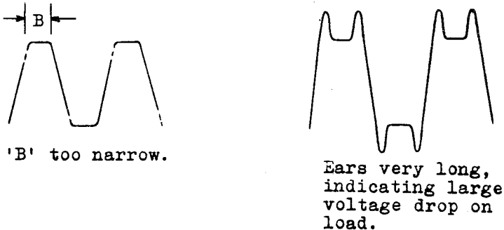
Fig 2. Characteristic waveforms under various circuit conditions.
