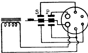
SERIES QE
