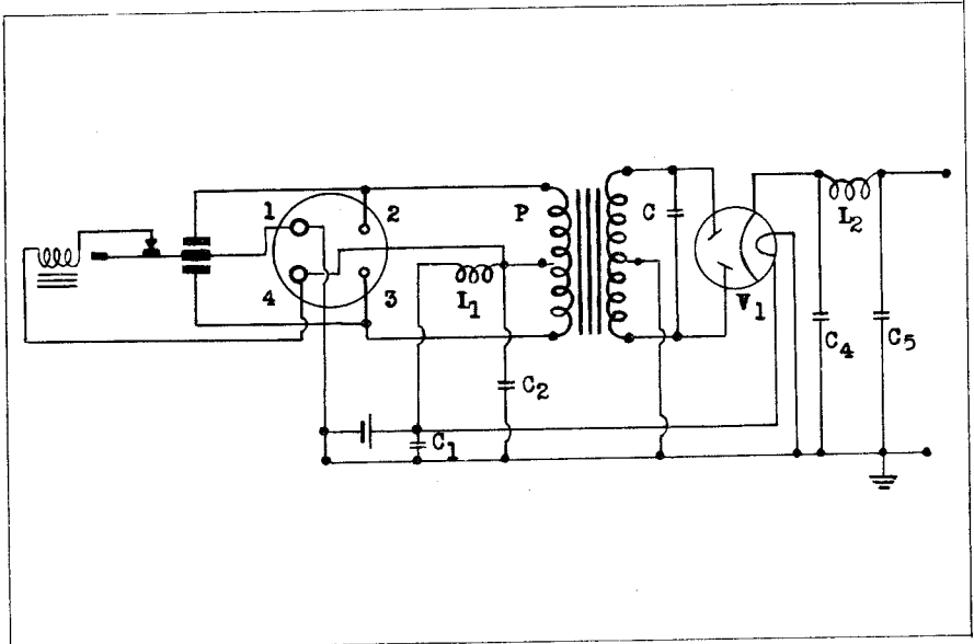
Fig 4. Circuit for simple power supply using Wearite non-synchronous vibrator Type NS with valve rectification, (excluding reservoir and smoothing circuit). When vibrator NSB is used omit connection to Pin No. 4.
