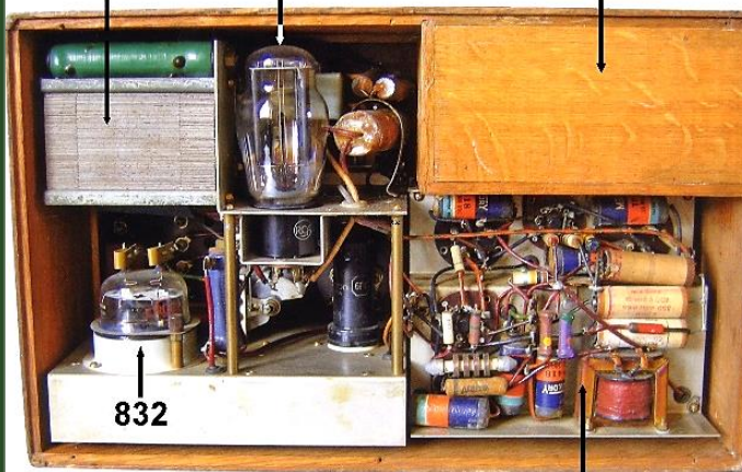
RECEIVER SECTION
